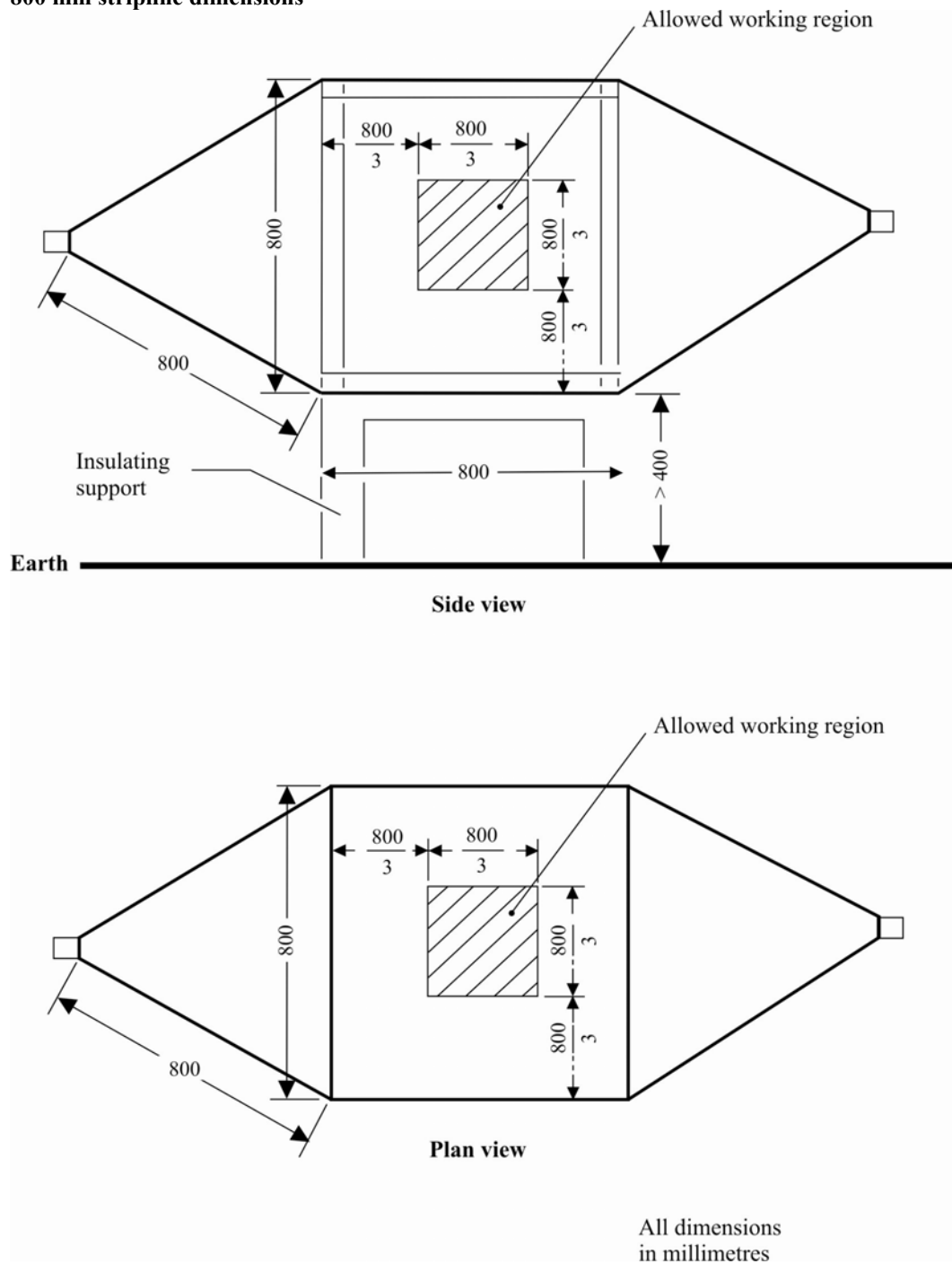
Figure 2 800 mm stripline dimensions
