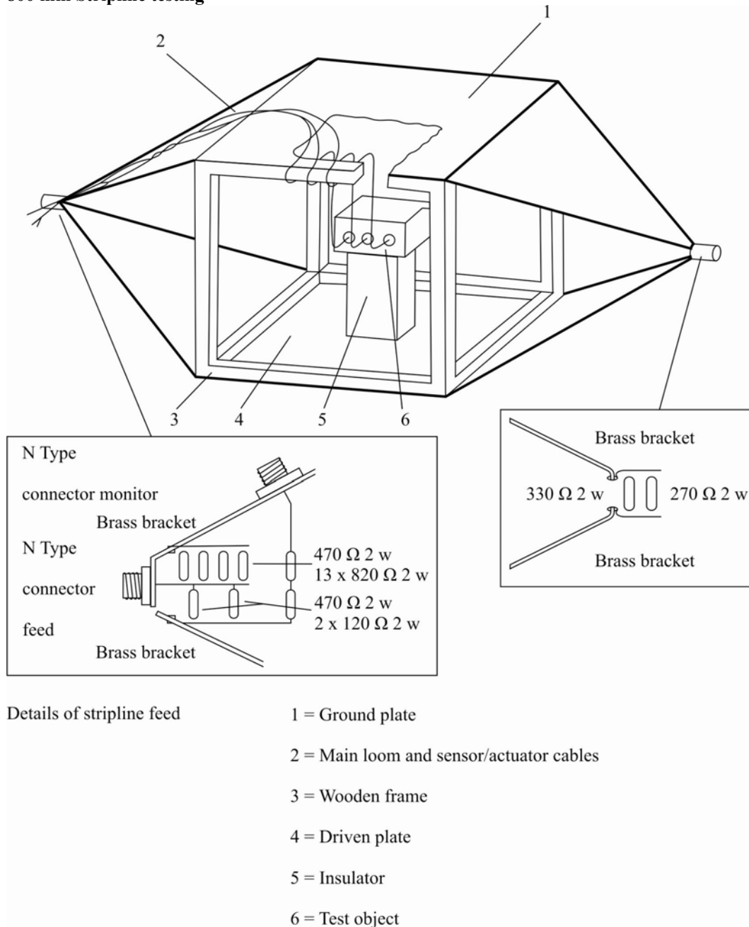
Figure 1 800 mm Stripline testing
